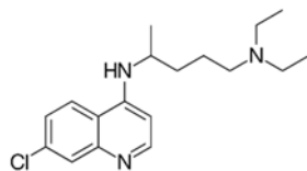
Figure 9. Chemical structure of Chloroquine.
